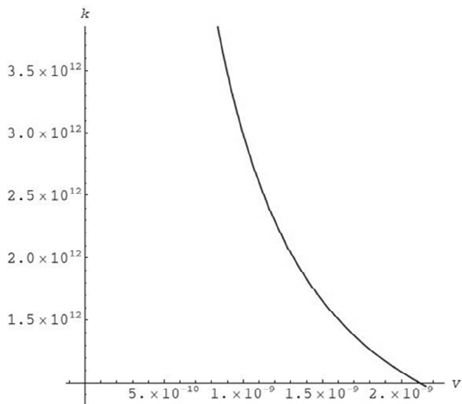
Figure 5: The ratio of the revolution frequency of the planet and the Kepler frequency of the rotation of the stars versus the scaled orbit radius \nu = \rho/R , for the example where the mass of the lighter star \mu = 1 and the heavier star \mu' = 100 (in the units of the mass of the Sun) and the interstellar distance R = 100 a.u. in the relativistic case.
