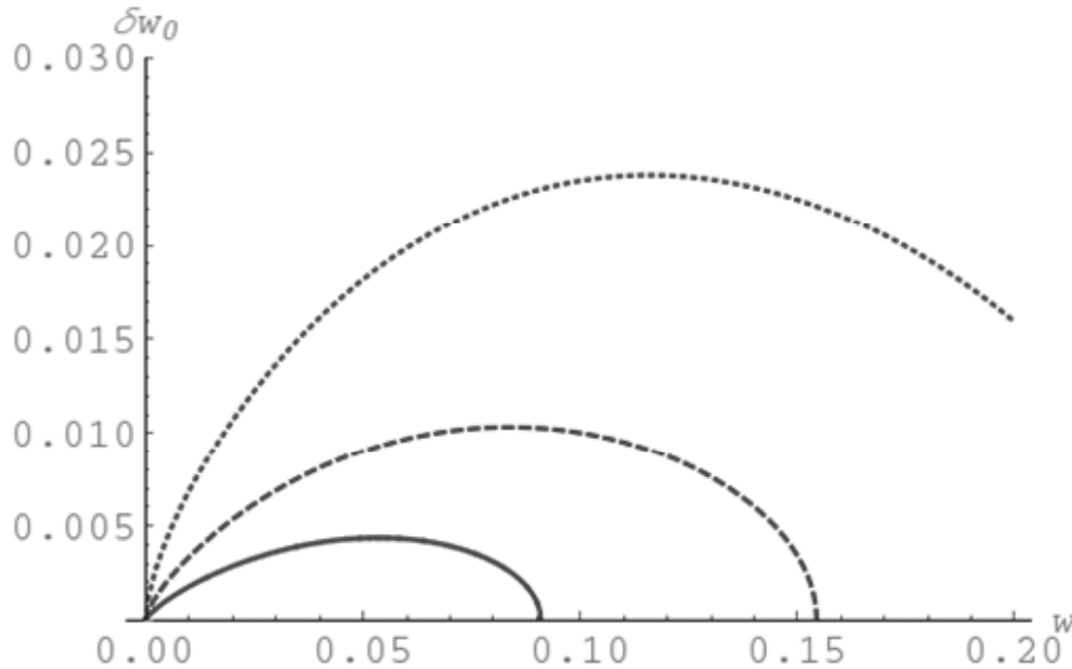
Figure 2: The scaled amplitude \delta w_0 of the oscillations of the planetary orbit along the interstellar axis versus the scaled projection w = z/R of the average plane of the planetary orbit on the interstellar axis, for three values of the ratio b of the stellar masses: b = 100 (solid line), b = 30 (dashed line), and b = 10 (dotted line).
