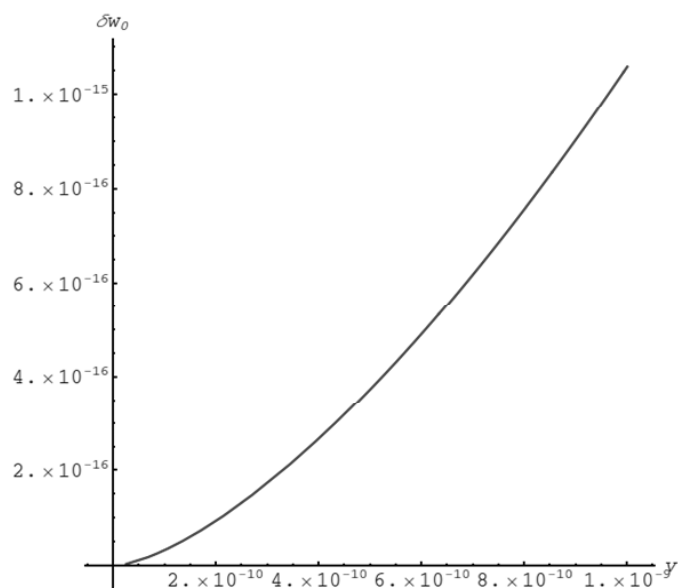
Figure 6: The scaled amplitude \delta w_0 of the oscillations of the planetary orbit along the interstellar axis versus the scaled orbit radius \nu = \rho/R for the example where the mass of the lighter star \mu = 1 and the heavier star \mu' = 100 (in the units of the mass of the Sun).
