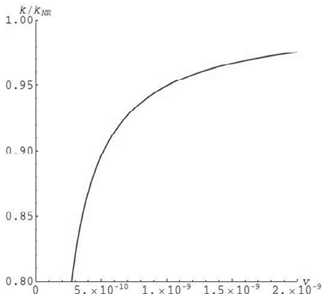
Figure 4: The ratio of the relativistic and non-relativistic k (which is the ratio of the frequencies of the revolution of the planet \Omega and the Kepler frequency \omega of the revolution of the stars about their barycenter) versus the scaled radius of the planetary orbit \nu = \rho/R , for the masses of the stars \mu = 1 and \mu' = 100 (in the units of the mass of the Sun) and the interstellar distance R = 100 a.u.
