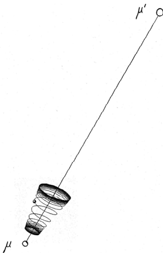
Figure 1: Sketch of the conic-helical motion of the planet in the model binary star system where the stars are stationary. We stretched the trajectory along the interstellar axis to make its details better visible.
