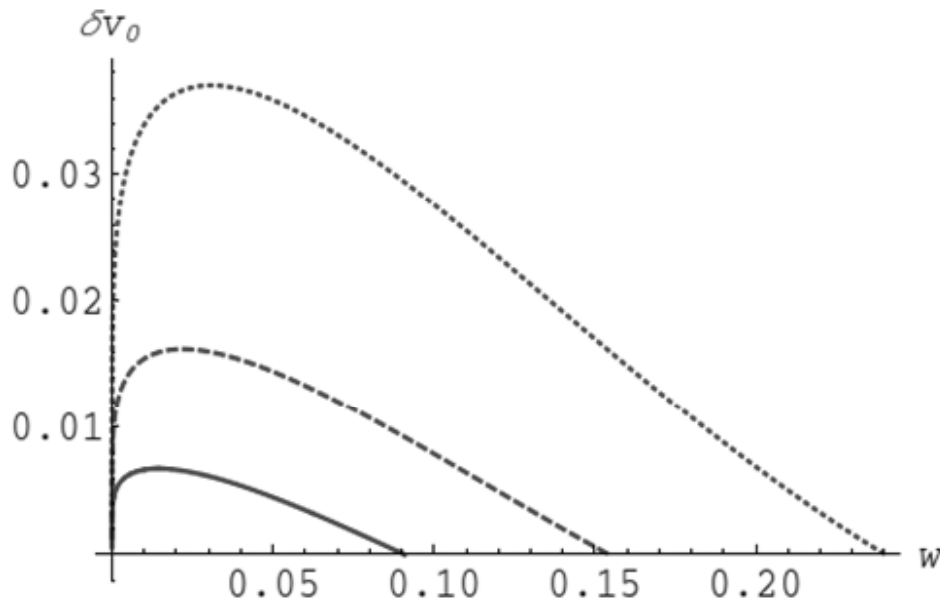
Figure 3: The scaled amplitude \delta v_0 of the oscillations of the planetary orbit along the radial coordinate versus the scaled projection w = z/R of the average plane of the planetary orbit on the interstellar axis, for three values of the ratio b of the stellar masses: b = 100 (solid line), b = 30 (dashed line), and b = 10 (dotted line).
